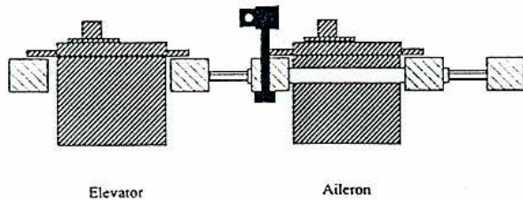
Combat Gremlin - Elevon mixer set up.
